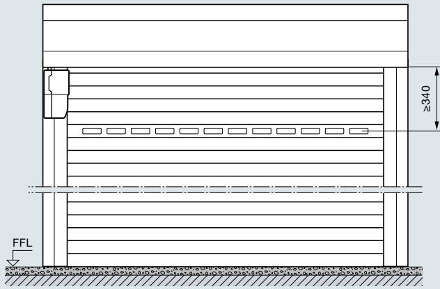
Internal roller garage door: Fitting behind the opening, view of fitting side
